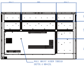
RM7502K * 螺絲類型：M8*25L
