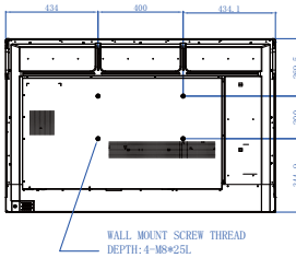
RM7502K * 螺絲類型：M8*25L
